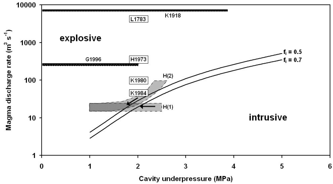
Figure 5. The critical discharge rate for eruptions on a 1.5 km fissure beneath 600 m of ice, plotted together with estimated magma discharge rates (normalised to fissure lengths of 1.5 km) and cavity underpressures for historical basalt fissure eruptions in Iceland, major 20 th century subglacial eruptions in Iceland and the Pleistocene tindar ridge of Helgafell. Symbols: L1783 - the Laki eruption; H1973 - the Heimæy eruption; K1980 - Krafla, July 1980; K1984 - Krafla, September 1984; G1996 - the Gjálp eruption; K1918 - the 1918 Katla eruption; H(1) - Helgafell, with a constant magma discharge rate and H(2) - Helgafell, with a waning magma discharge rate. The arrows indicate the inferred change in underpressure during the Helgafell eruption, from c. 2.5 to 1 MPa [Schopka et al. , 2006].
