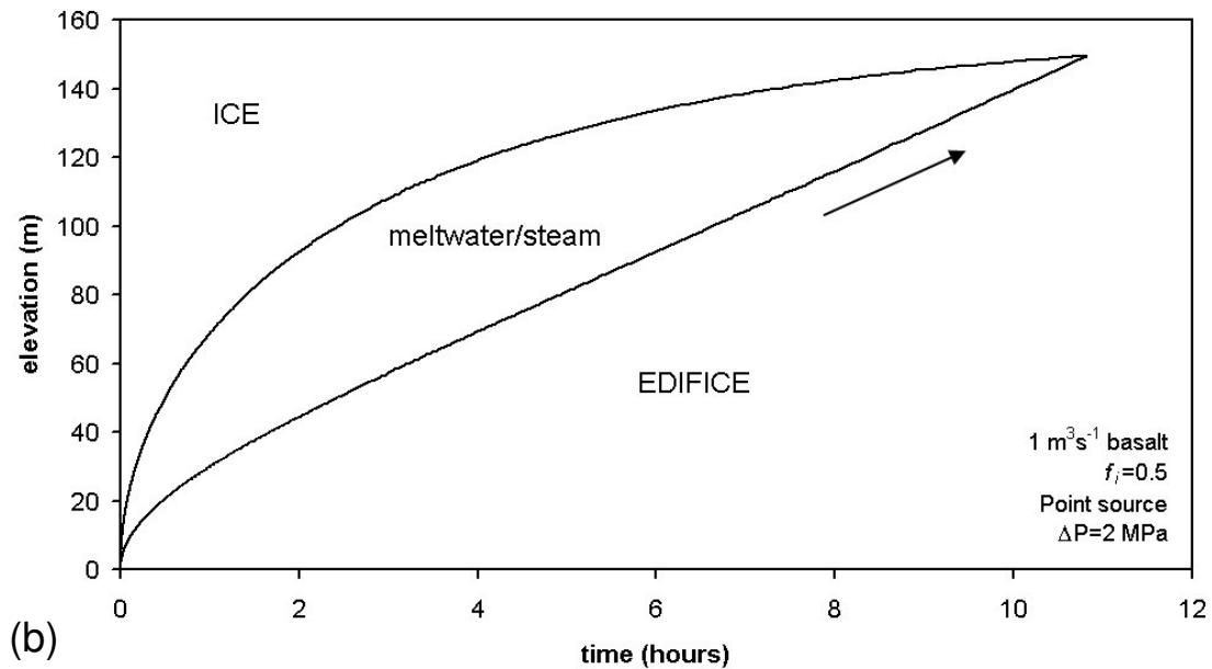
Figure 3. Graphs showing the position of the cavity roof and top of the edifice during two eruptions from a point source beneath 600 m of ice. (a) At a high magma discharge rate ( 100 \text{ m}^3 \text{ s}^{-1} ), the cavity size increases much more quickly than the edifice, creating a significant depth of meltwater/steam in which hydroclastic fragmentation can occur. (b) At a lower magma discharge rate, closure of the cavity is more important and the edifice soon completely fills the cavity (arrow), leading to an intrusive style of eruption. Note that the timescale in (b) is much longer than in (a).
