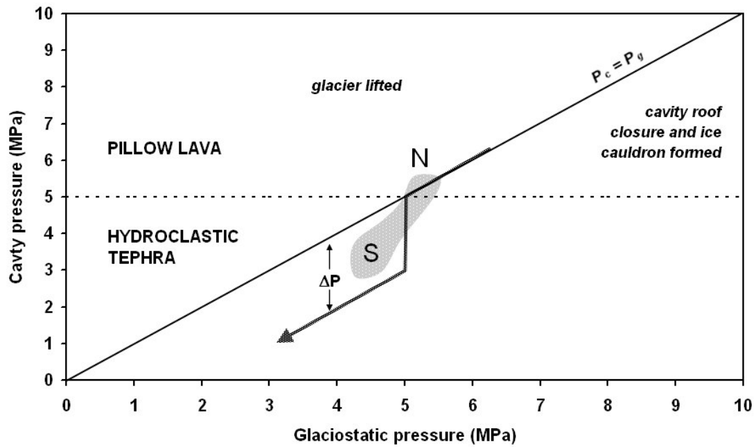
Figure 2. A diagram indicating the possible relationship between cavity pressure ( P_c ) and glaciostatic pressure ( P_g ) during subglacial eruptions. To the left of the diagonal line P_c = P_g , the glacier is lifted; to the right, cavity underpressure (indicated by \Delta P ) leads to cavity roof closure and ice surface deformation. The shaded area indicates the probable pressure conditions during the Gjalp eruption [from Guðmundsson et al. , 2004], with the northern (N) and southern (S) ends of the fissure indicated. The arrow indicates the inferred pressure path during an eruption that starts with pillow effusion but becomes explosive as roof thinning reduces the cavity pressure to less than 5 MPa.
