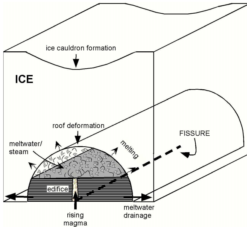
Fig. 1. A cartoon showing a fissure eruption at the base of a glacier. A hemicylindrical cavity has been melted above the fissure and a flat-topped volcanic edifice is emplaced within it. Any space above the edifice is filled by meltwater, possibly with some steam, which provides space for explosive magma-water interaction. Meanwhile, the cavity roof closes towards the edifice, forming an ice cauldron on the glacier surface. Meltwater drains away from the eruption site at the glacier base.
