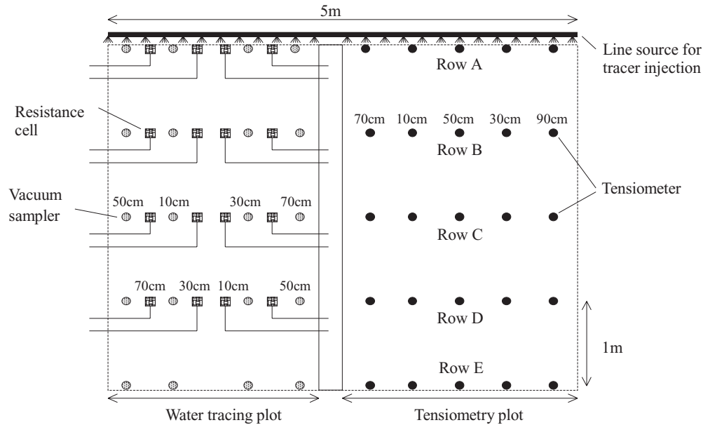
Figure 2. Layout of instrumentation within the experimental hillslope
