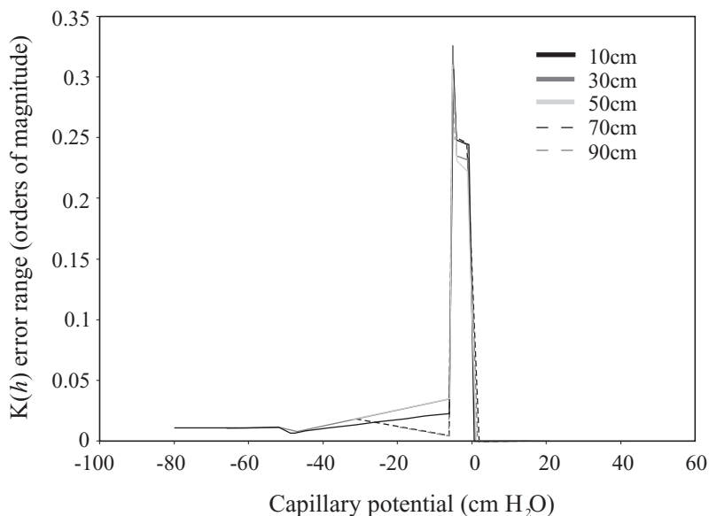
Figure 5. Error range of depth-specific hydraulic conductivity resulting from \pm 0.5 cm H_2O capillary potential error
