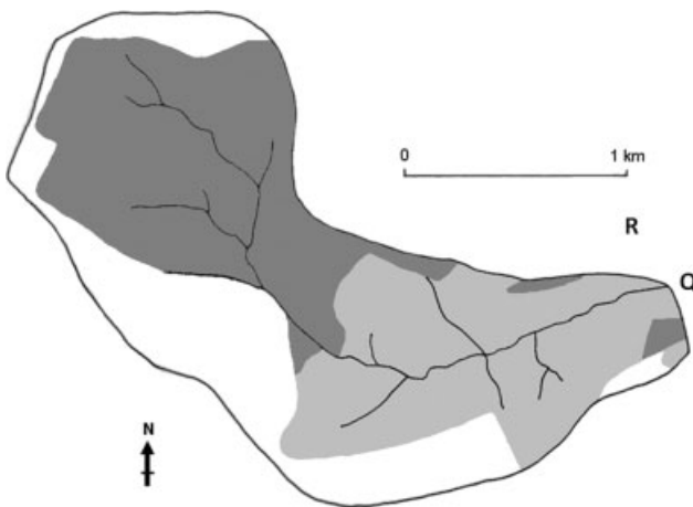
Figure 3. Map of the Afon Hore catchment showing the clear-felled forest coupes within the lower reaches (modified from Roberts and Crane, 1997) that is located within the 8.7 km 2 Severn experimental catchment on the Plynlimon massif, mid-Wales, UK (52.4°N, 3.7°W). The solid line shows the boundary of the Afon Hore catchment and the stream channel. The dark shading shows the extent of forest inside the Afon Hore catchment, while the light shading shows the area of clearfelling between December 1985 and October 1987. Symbol Q shows the location of the Afon Hore flume and R the location of the Moel Cynnedd raingauge
