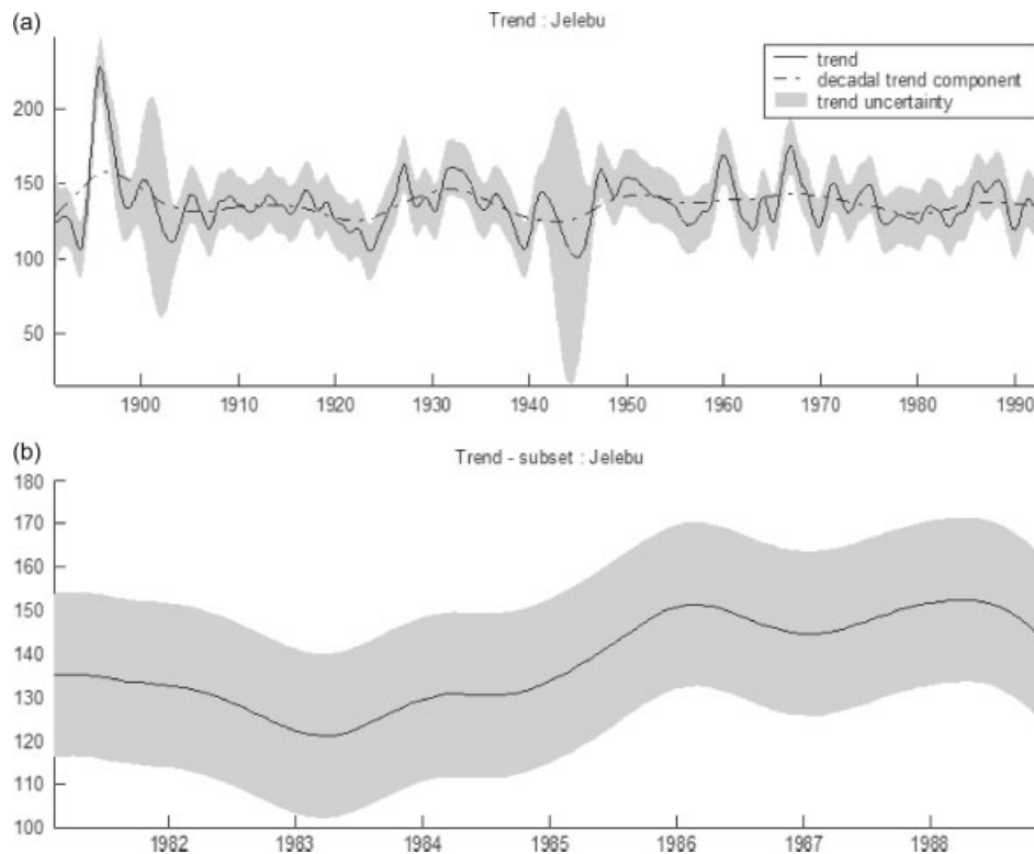
Figure 6. UC-DHR identified inter-annual trend in the Jejebu rainfall from 1891 to 1992 (solid line) and uncertainty band, where (a) shows the whole period, while (b) shows only the period coincident with the Bukit Berembun catchment studies. The x -axis is the year, the y -axis is the rainfall (mm/month) and the shading encompasses the standard deviation (SD)
