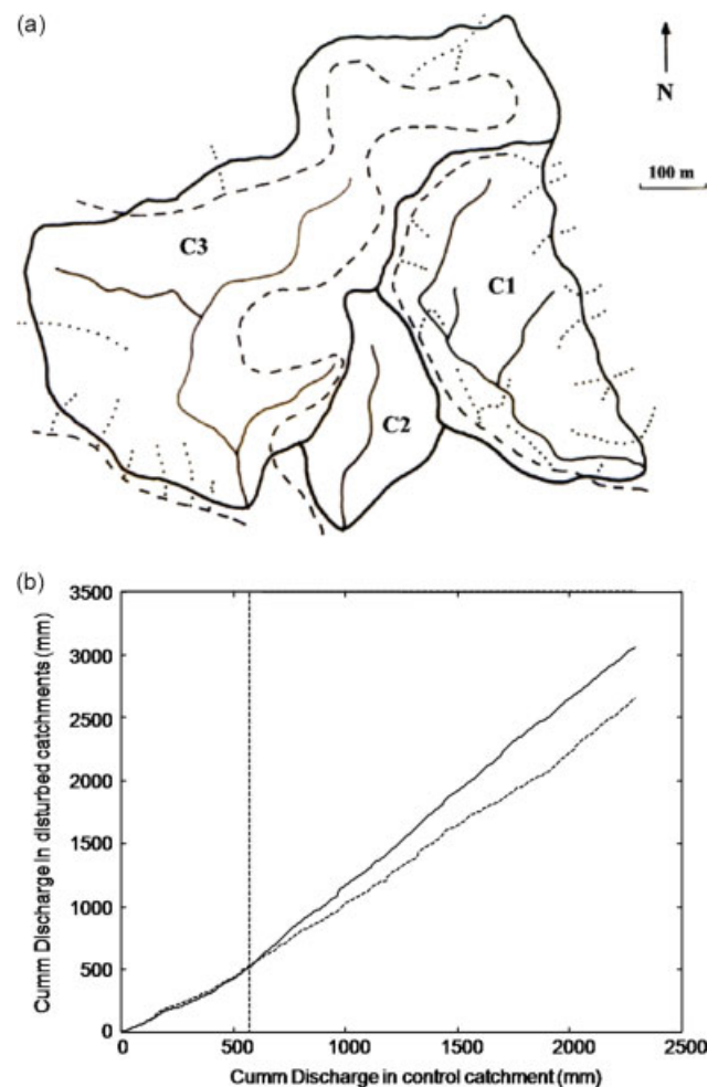
Figure 1. The Bukit Berembun experimental study at 2°46'N, 102°6'E in Negri Sembilan state, Peninsular Malaysia: (a) a map of the Bukit Berembun C1, C2, and C3 catchments, where the catchment divides are shown with a broad solid line, streams with a fine solid line, roads with a dashed line and skid trails with a dotted line, and (b) the double mass curve of streamflow for the conventionally-logged (C1) catchment against that of the control (C2) shown with a solid line and the 1 : 1 relationship with a broken line
