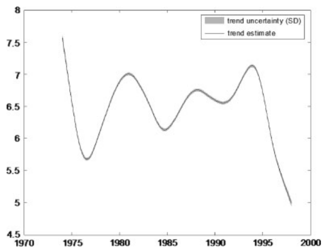
Figure 11. UC-DHR identified inter-annual trend in the Moel Cynnedd rainfall from 1974 to 1997 (solid line) and uncertainty band. The x-axis is the year, the y-axis is the fortnightly rainfall (mm/d) and the shading encompasses the standard deviation (SD)
