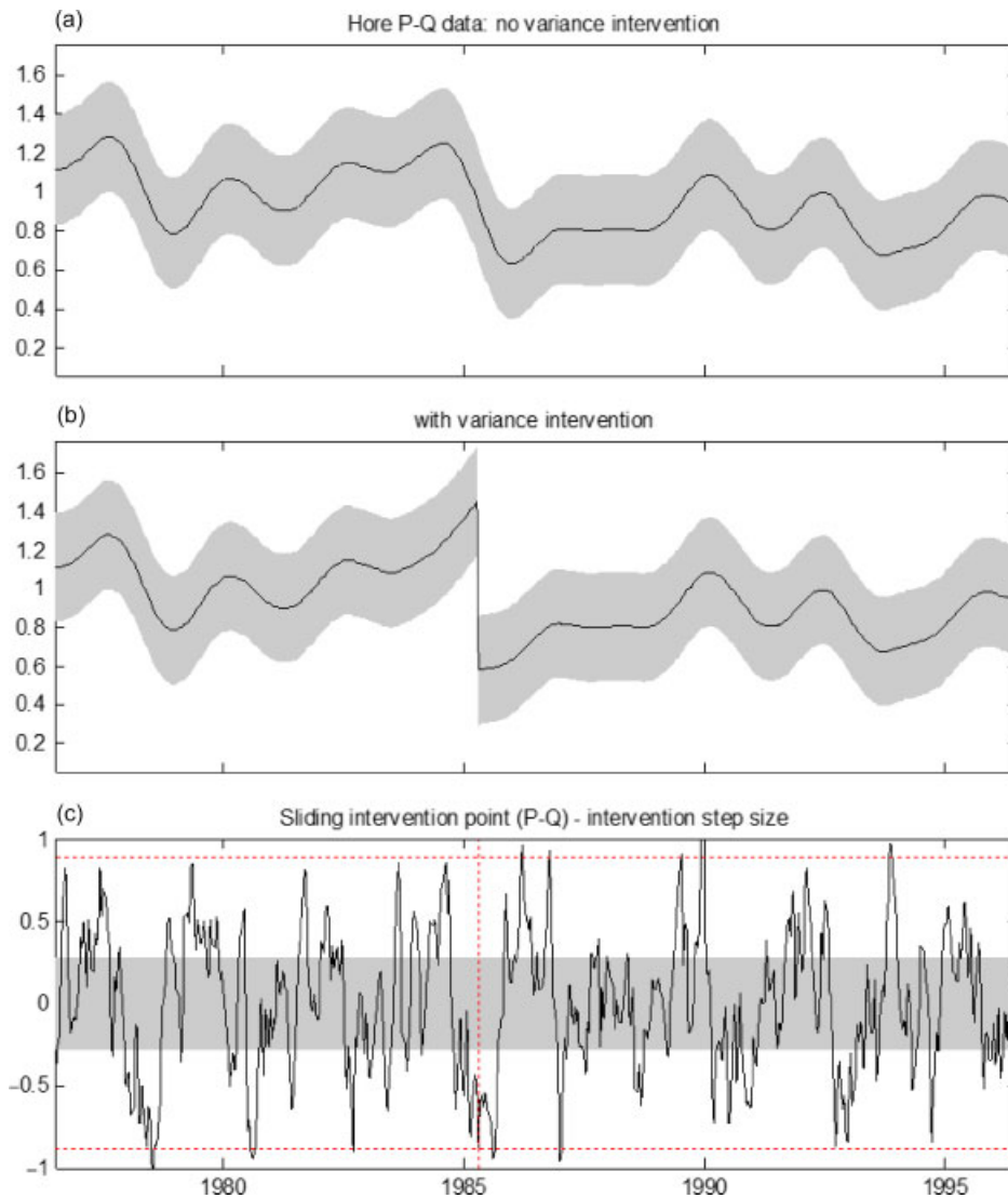
Figure 10. UC-DHR identified inter-annual trend in the Afon Hore P-Q time-series for (a) without Variance Intervention, (b) with Variance Intervention at the start of clearfelling in 1985, and (c) the magnitude and change in the modelled step change in the Afon Hore P-Q when the UC-DHR model was run with an intervention point placed at 289 locations in the time series (i.e. each month of record). The x-axis is the year, the y-axis is the fortnightly P-Q (mm/d) and the shading encompasses the standard deviation (SD)
